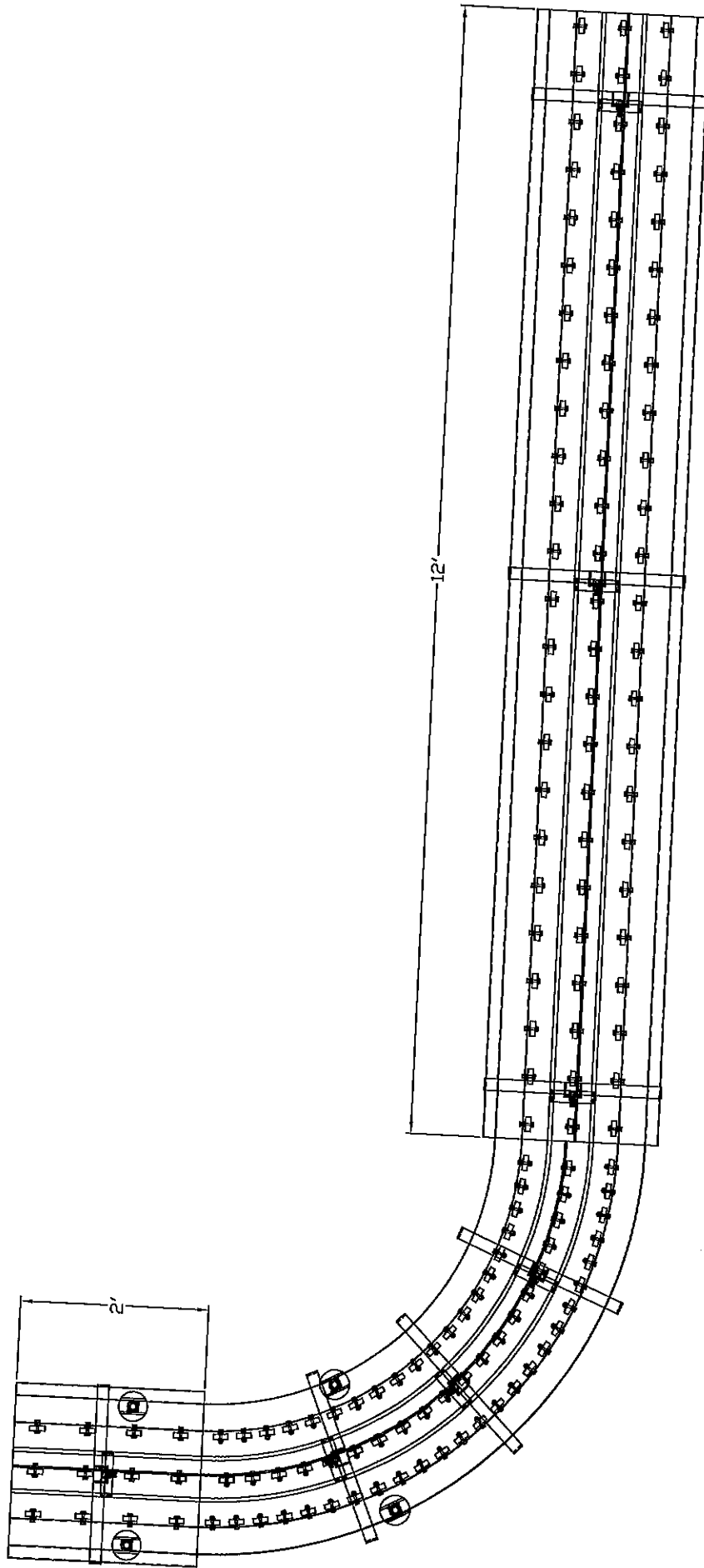
C121241-X99 PLAN VIEW
